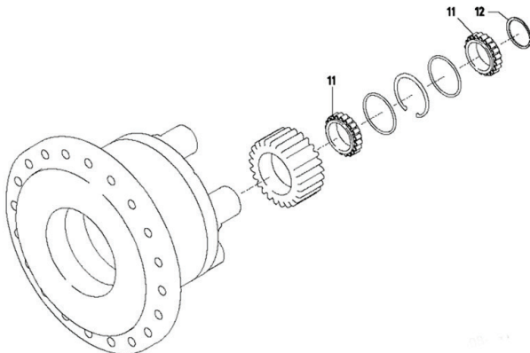
R988091014 - GFT 8190 - bearing main stage
