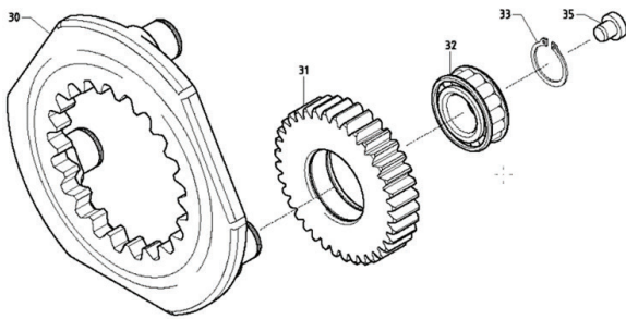
R988091083 - GFT 8190 - pre-stage (assembled)
