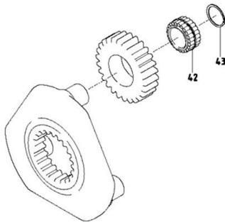
R988091014 - GFT 8190 - bearing main stage
