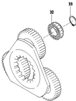
R988091034 - GFT 8190 - bearing 2nd pre-stage
